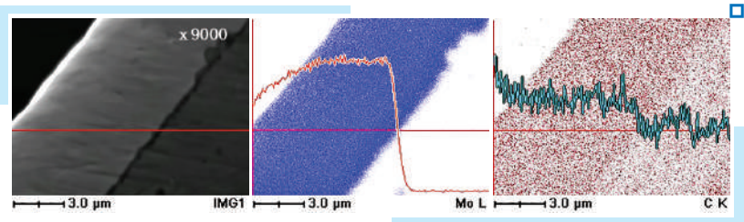
Fig. 3.11 Appearance of Avinit D/P 200 coating (Mo-C system based) in the in-line analysis mode. The coating thickness is ~6 μm
