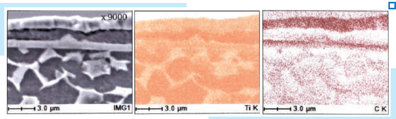
Fig. 3.10 Appearance of Avinit D/P 100 coating (Ti-C system based) (cross-section) in the mapping mode of the coating area. The higher element content corresponds to the more intense coloring. The coating thickness is ~3.5 μm
