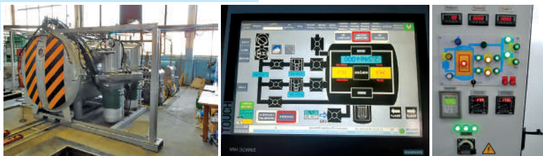
■ Fig. 4.9 Upgraded automated vacuum-thermal installation for diffusion welding and thermal treatment with horizontal loading, forced gas cooling of the melting charge
