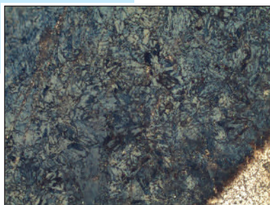
■ Fig. 3.36 The microstructure of the nitrided layer on 34NiCrMoV14-5 steel ( \times 500 )
