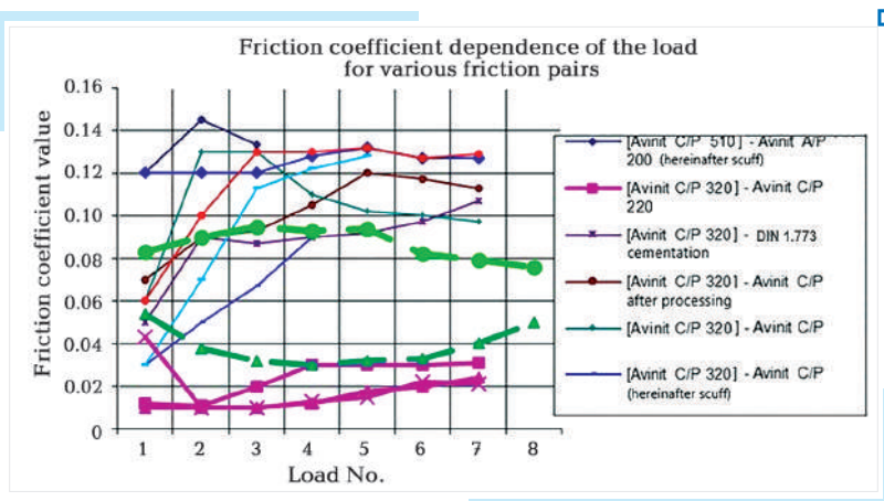
□ Fig. 3.22 Friction factors
