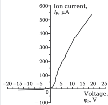
■ Fig. 3.33 Typical volt-ampere characteristic (VAC) of a probe at a pressure of 1.2 \cdot 10^{-2} Torr, using which the plasma parameters (ion current, plasma density, electron temperature, degree of flow ionization) were calculated
