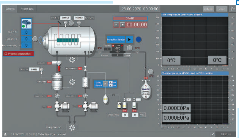
Fig. 2.7 Avinit V gas-phase mnemonic diagram
