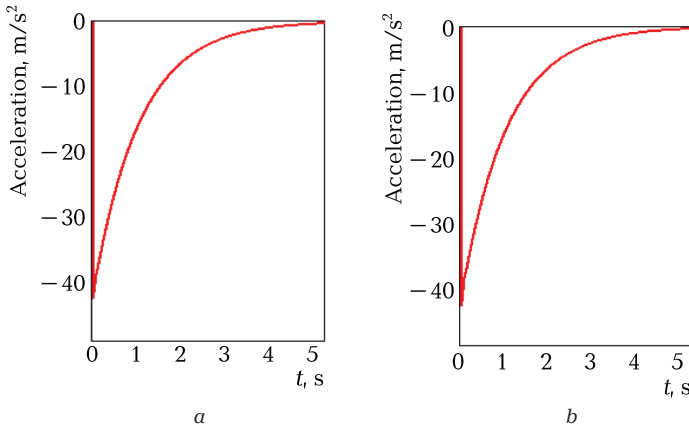
Fig. 3.20 Acceleration acting on the bearing structure of an articulated flat wagon: a – the first section of the flat wagon from the side of the action of the longitudinal force; b – the second section of the flat wagon from the side of the action of the longitudinal force
