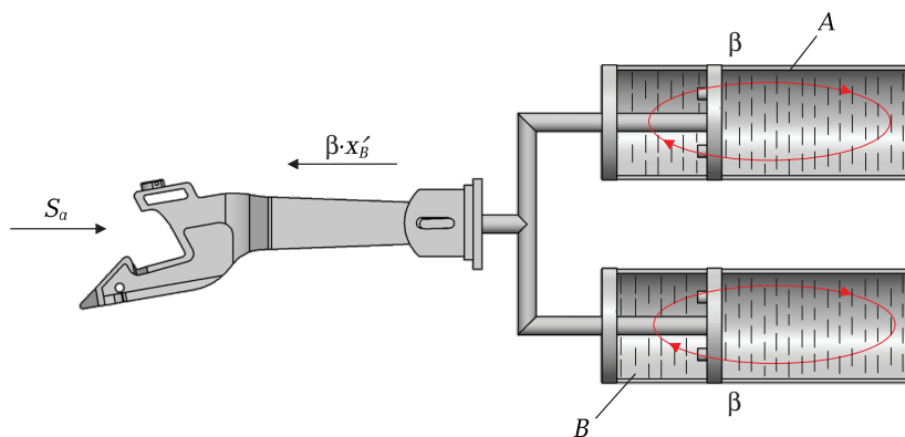
Fig. 2.10 Operation scheme of the harness concept of a gondola wagon
