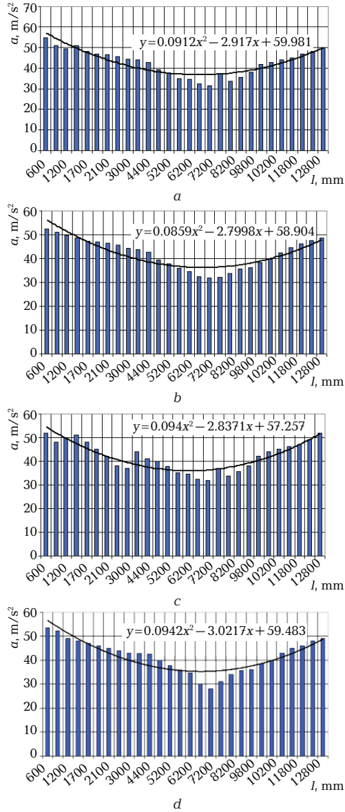
Fig. 2.7 Distribution of accelerations along the length of the center beams of the frames of railway wagons under the action of the longitudinal impact force on the adapter: a – flat wagon; b – gondola wagon; c – covered wagon; d – hopper wagon
