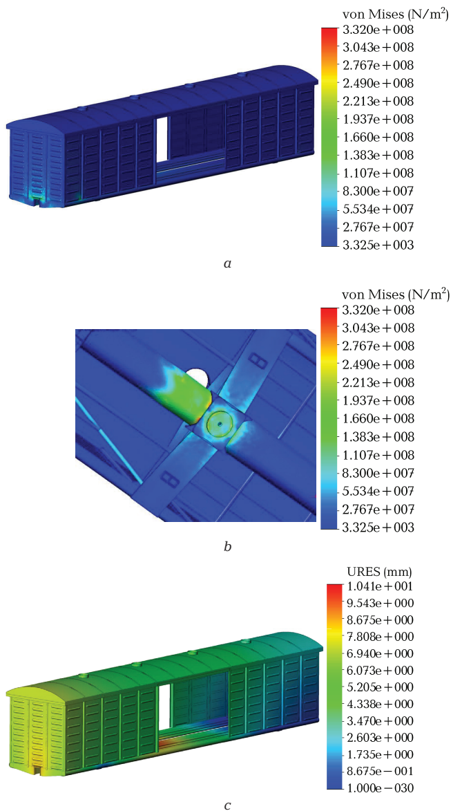
Fig. 1.23 The results of the strength calculation of the body of a covered wagon with an improved design under the conditions of I design mode (impact): a – stress state (side view); b – stress state (bottom view); c – displacement in nodes
