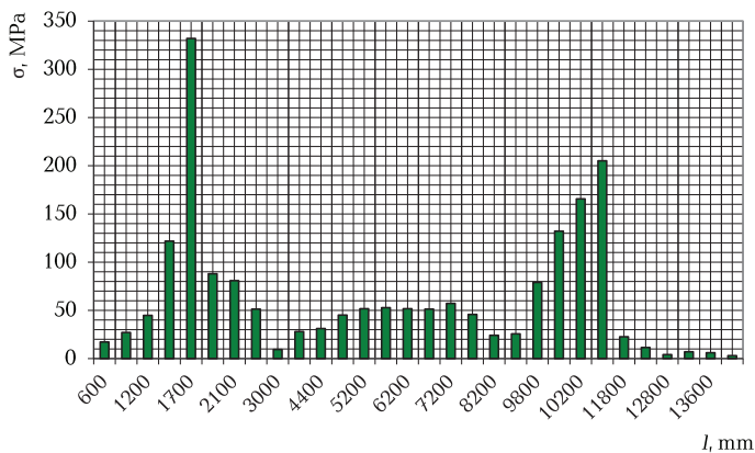
Fig. 1.24 Distribution of equivalent stresses along the length of the center beam under the I design mode (impact)
