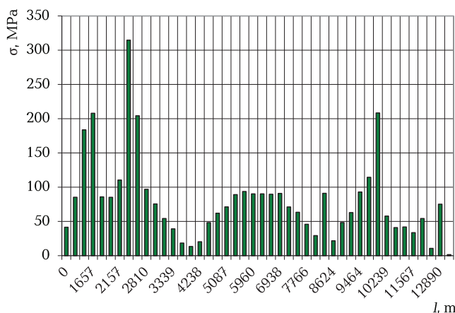
Fig. 1.9 Distribution of equivalent stresses over length of the center beam
