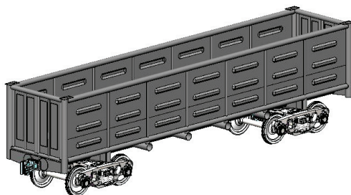
Fig. 1.19 Gondola wagon made of round pipes
