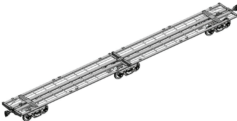
Fig. 3.7 Articulated flat wagon made of pipes of circular cross-section
