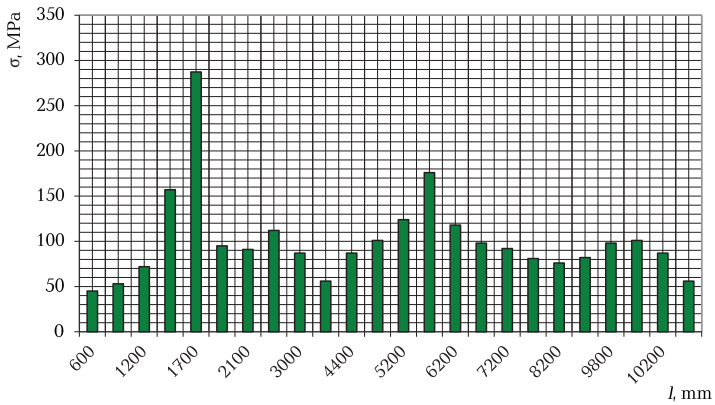
Fig. 1.30 Distribution of stresses along the length of the center beam of the hopper wagon
