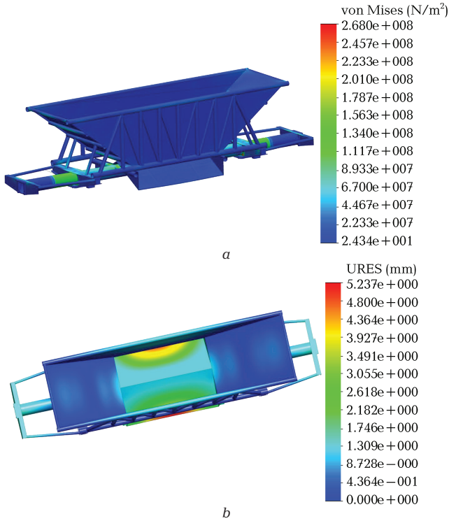
Fig. 1.29 The results of the strength calculation of the hopper wagon body of an improved design in the conditions of the design mode (impact): a – stressful state; b – movements in nodes
