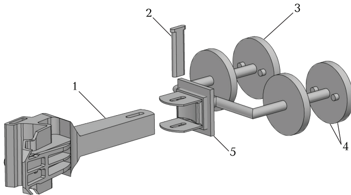
Fig. 2.8 Concept of automatic coupler harness: 1 – automatic coupler body; 2 – wedge; 3 – piston; 4 – throttle valves; 5 – thrust bar
