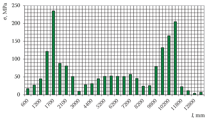
Fig. 1.18 Distribution of equivalent stresses along the length of the gondola wagon (in the lower zone of the pipe)
