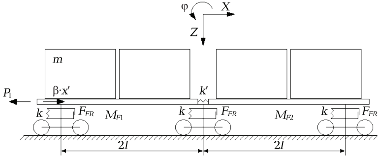
Fig. 3.19 Design diagram of an articulated flat wagon
