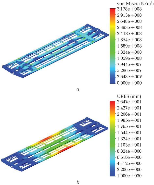
Fig. 1.8 The results of the strength calculation of the platform wagon of the improved design in the conditions of the I design mode (impact): a – stressful state; b – movement in nodes
