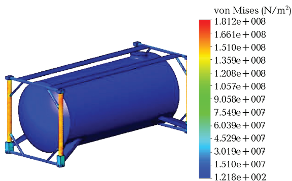
Fig. 1.37 Diagram of statistical nodal loads when stacked in 4 tiers
