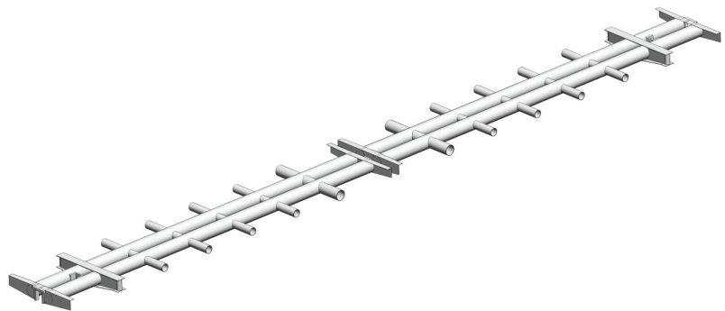
Fig. 3.14 Frame of an articulated gondola wagon
