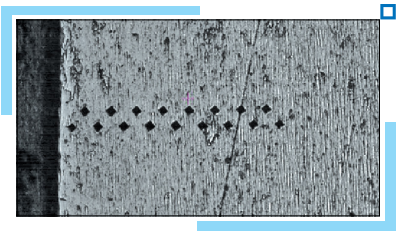
Fig. 3.32 Appearance of microhardness measurements imprints. Side No.2
