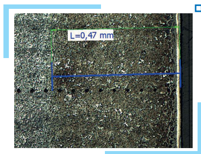
Fig. 3.21 Depth of nitrided layer
