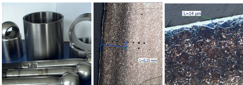
Fig. 4.1 Duplex technology of Avinit on turbine steam distribution elements
