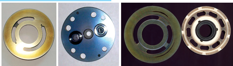
■ Fig. 3.37 Spools of hydraulic units with Avinit nanocoatings
