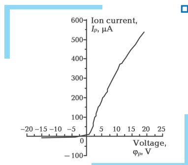
■ Fig. 3.14 Volt-ampere characteristic of a double arc discharge probe
