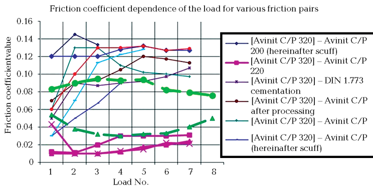
Fig. 3.12 Friction factors
