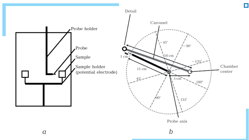
Fig. 2.2 Location of the Langmuir probe in the vacuum chamber of the Avinit installation: a – cross-sectional side view; b – a top view
