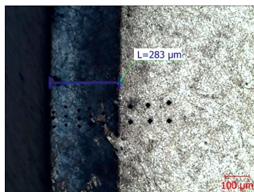
Fig. 3.25 Imprints of microhardness measurements (etched polished)
