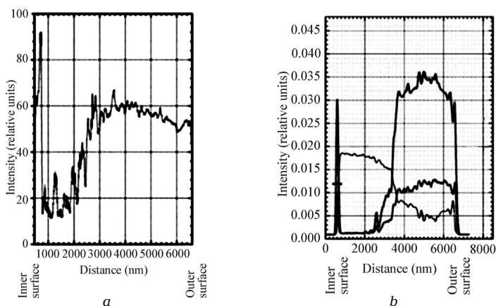
Fig. 3.7 Distribution of characteristic X-ray radiation of element atoms in Avinit C 320 coating: a – at. % Ti; b – at. % Al
