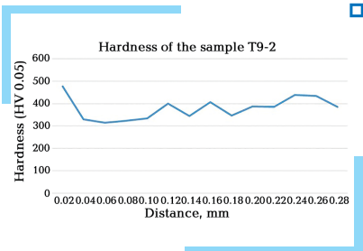
Fig. 3.30 The magnitudes of change in the hardness of the nitrided layer
