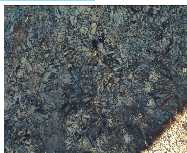
■ Fig. 3.17 The microstructure of the nitrided layer on 34NiCrMoV14-5 steel (×500)
