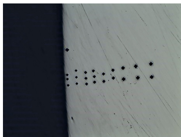
Fig. 3.24 Imprints of microhardness measurements (unetched polished section)
