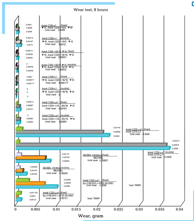
Fig. 3.13 Generalized tribological test results
