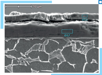
■ Fig. 3.41 The structure of the nitrided layer. Depth of the nitrided layer 0.2 mm. Microhardness H_\mu = 730\text{--}830 . Avinit coating layer thickness 1-2- \mu\text{m} , H_\mu = 3000
