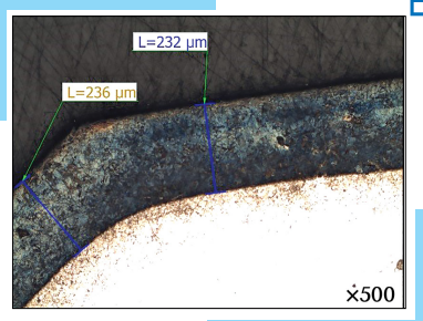
Fig. 3.23 The nitrided layer depth
