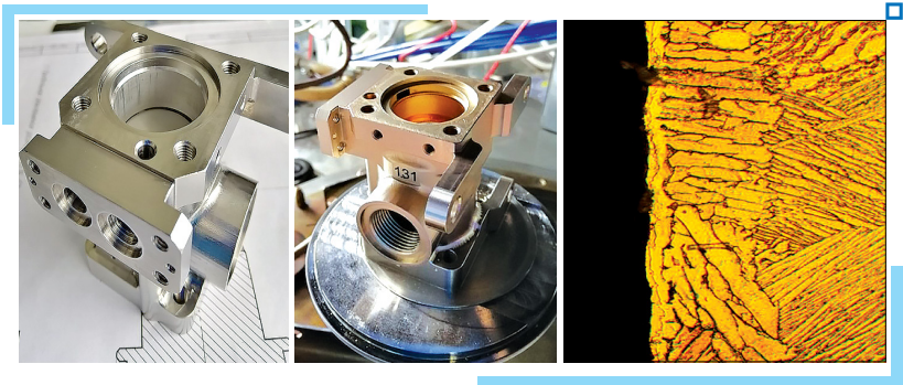
Fig. 3.33 Housing from DIN 3.7165 titanium alloy. The structure of the nitrided layer on the inner cylindrical part of the housing surface
