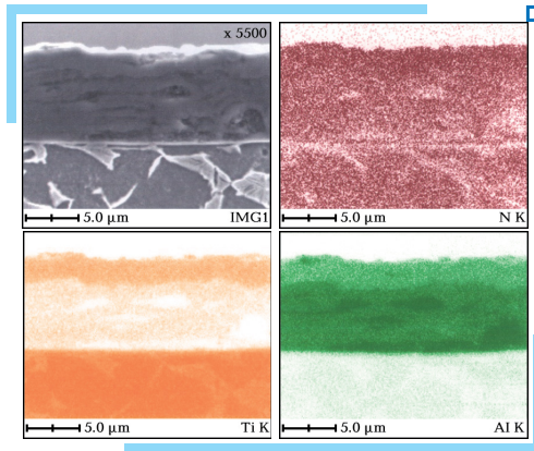
□ Fig. 3.8 Appearance of a covering of Avinit C/P 310 (cross section) in the mode of mapping of a site of a coating
