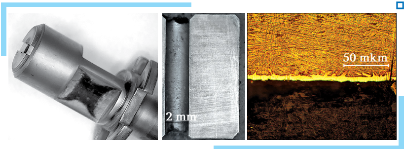
Fig. 3.34 Slide valve. Structure of nitrided layers on slide valve surface
