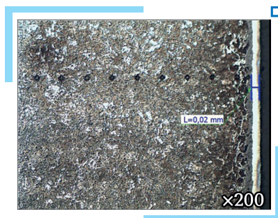
Fig. 3.22 Microstructure in the zone of the nitrided layer
