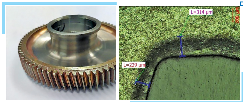
Fig. 3.39 Full-size high-precision gear, made using duplex technology Avinit. Depth of the nitrided layer 0.3\text{ mm} . Microhardness H_{\mu} = 730\text{--}930 . Avinit coating layer thickness 1\text{--}2\text{ }\mu\text{m} , H_{\mu} = 3000
