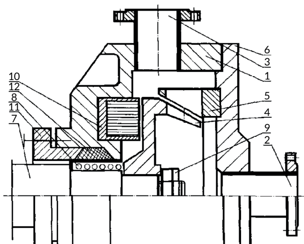
Fig. 3.15 Rotor-pulsating device with a vibrating rotor
