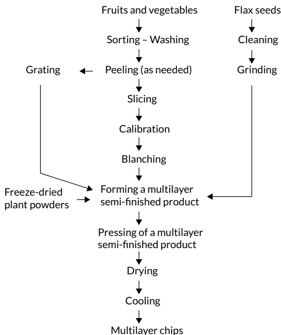
Fig. 5.1 Flowchart of technology of multilayer fruit and vegetable chips
