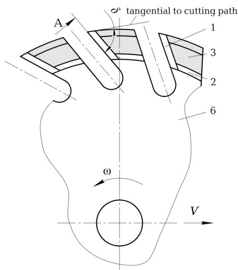
Fig. 3.6 A fragment of the lateral surface of the working body with the developed elements of differential design
