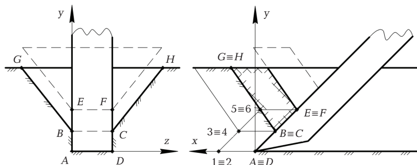
Fig. 3.1 Differentiated scheme for determining the power and energy parameters when cutting soils
