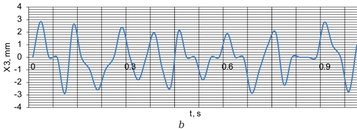
Fig. 4.6 Vibrograms of mass oscillations of the crusher during its operation with material ( \omega = 104.667 rad/s, F = 4111 N, c_2 = 219052 N/m): a – movement of the second mass; b – movement of the third mass
